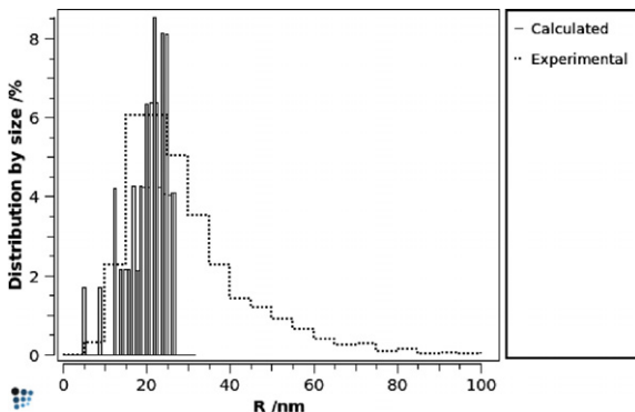
Fig. 6. Comparison between carbide distribution determined experimentally (dotted line) and calculated (bars) for alloy F82H after thermal aging at 250 °C.
