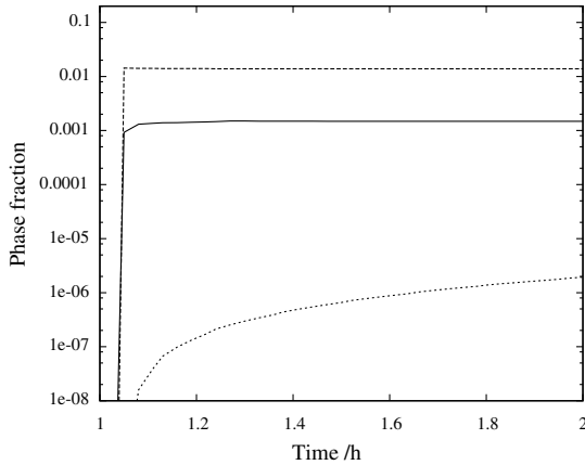
Fig. 3. Evolution of the precipitate phase percentage in alloy JLF-1 during the tempering stage of the As Manufactured treatment. Solid line corresponds to MX precipitates; dashed line to M_7C_3 and dotted line to M_{23}C_6 .
